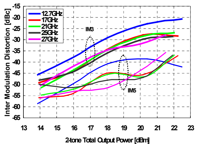
IMD vs. Output Power
