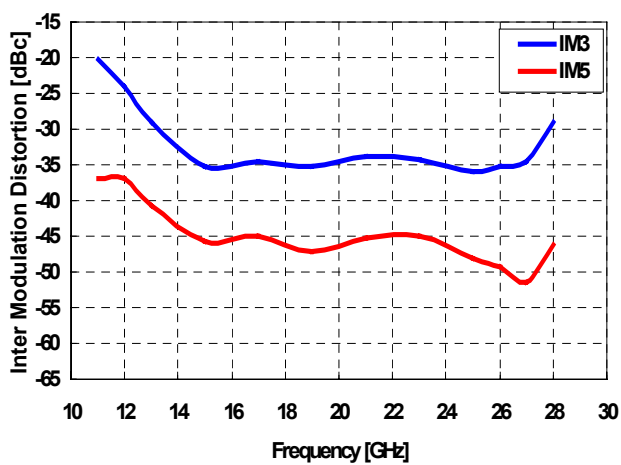
IMD vs. Frequency @VDD=6V, IDD(DC)=300mA, Pout=15dBm S.C.L
