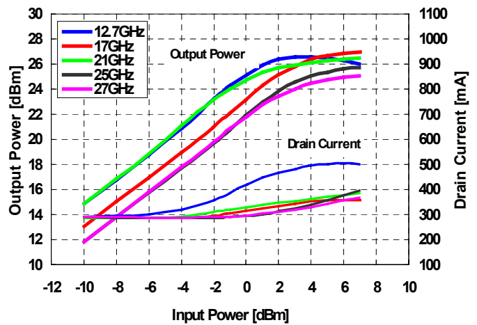
Output Power, Drain Current vs. Input Power
