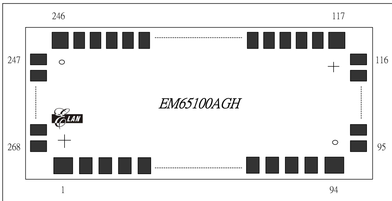
Figure 1. Pin configuration
