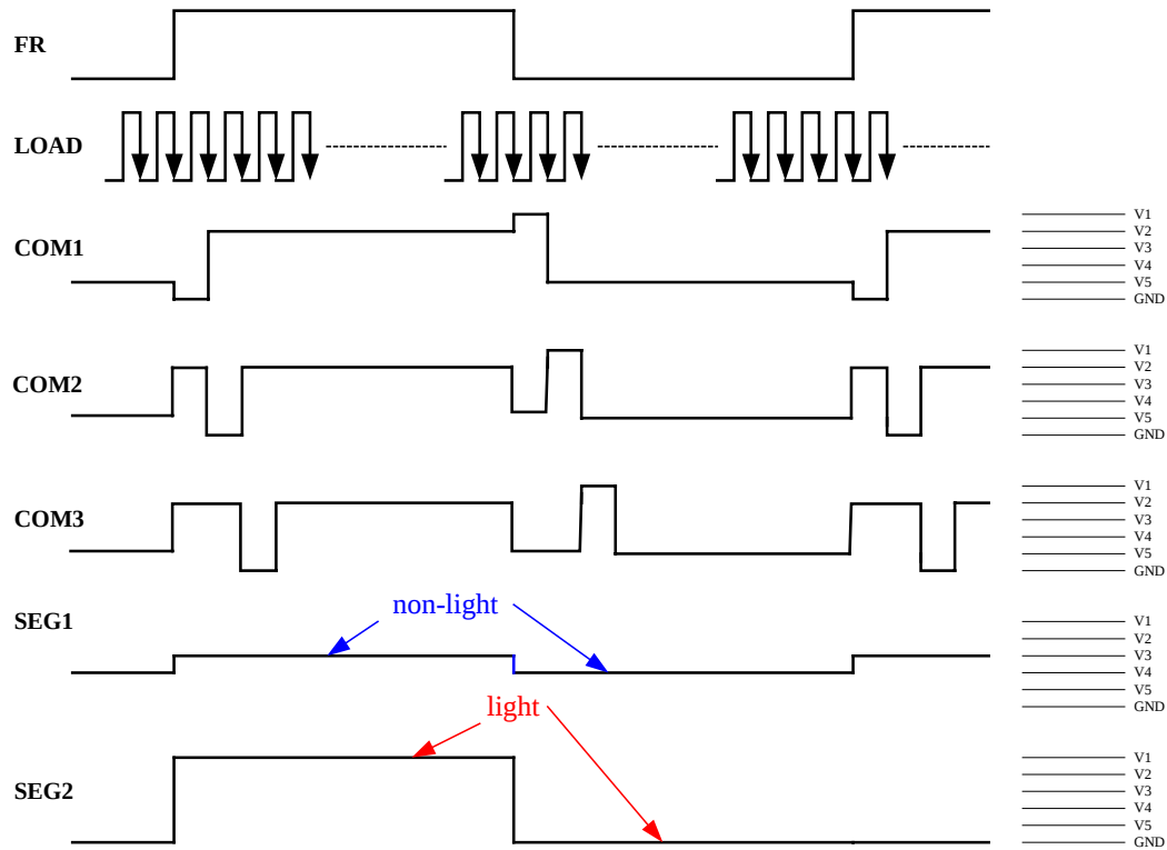
FIG. 9 LCD Waveform
