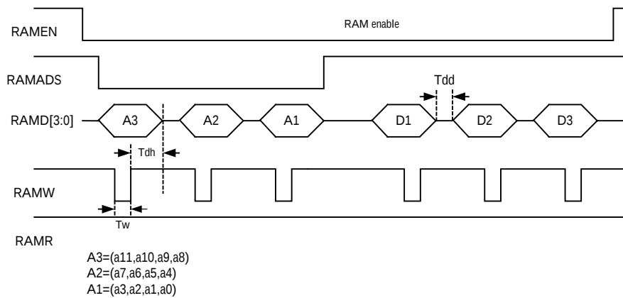
FIG. 3 LCD RAM write mode for 4-bit bus
