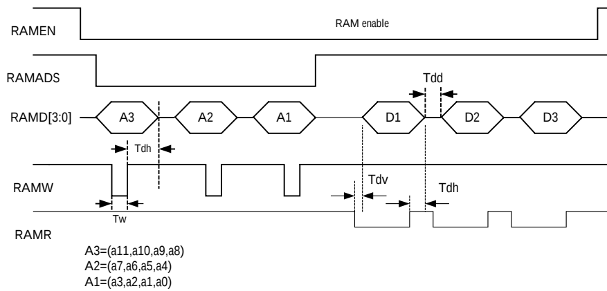
FIG. 5 LCD RAM read mode for 4-bit bus
