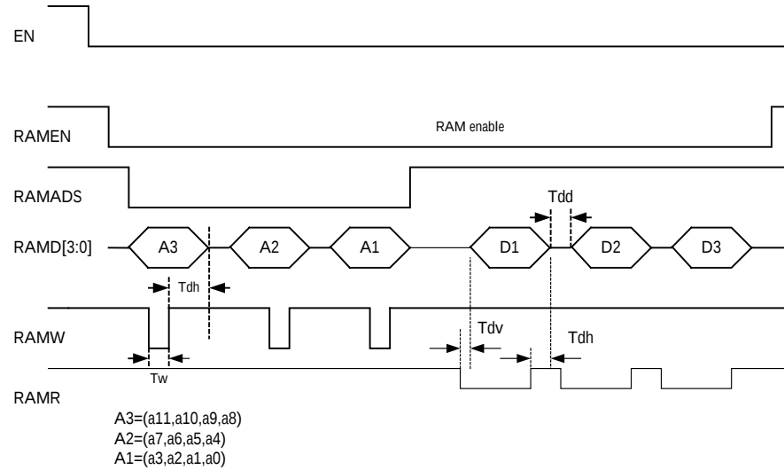
FIG 16 LCD RAM read mode
