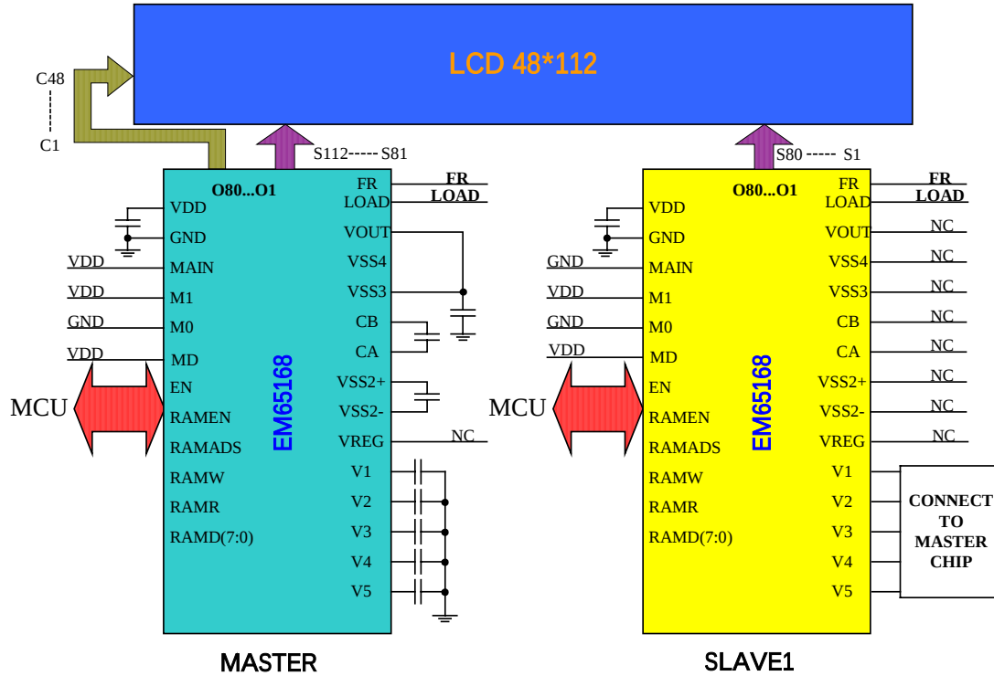
FIG. 20 48common*112segment application circuit
