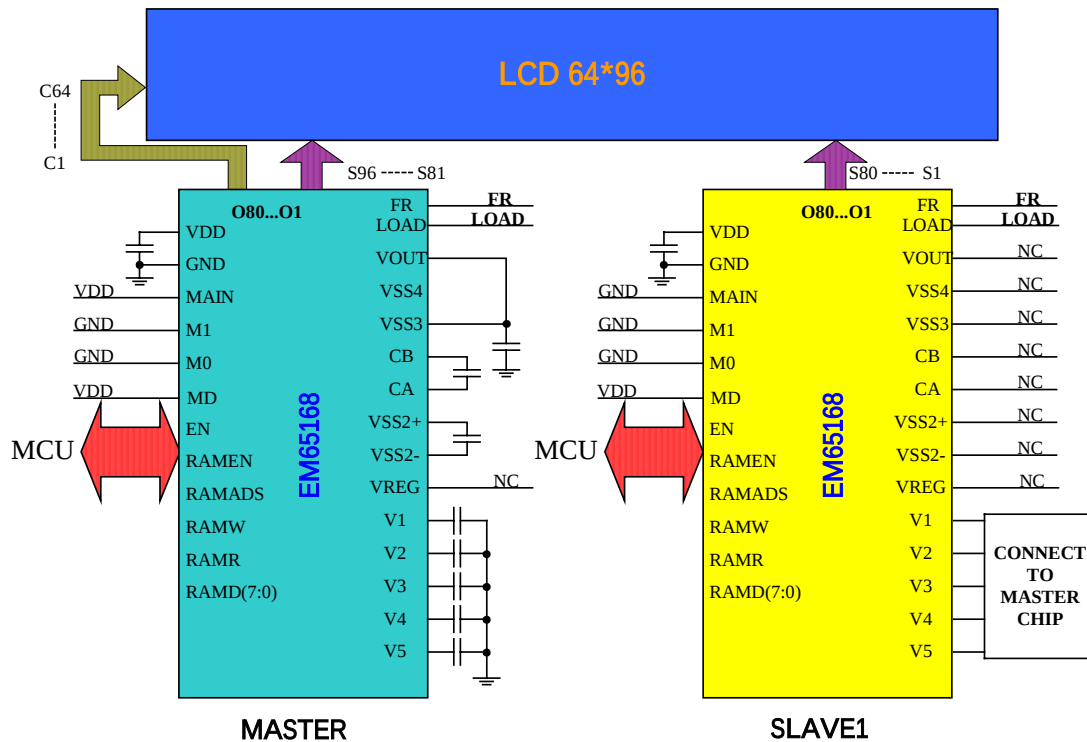
FIG. 21 64common*96segment application circuit
