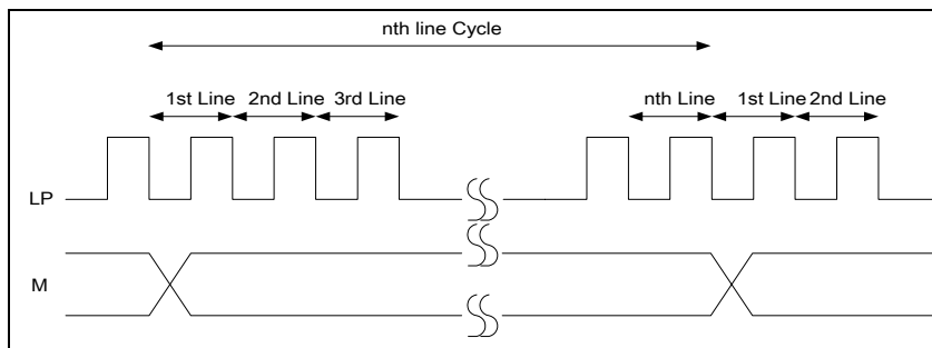
Figure 8-2b NLINE = "1" Alternate Timing Diagram
