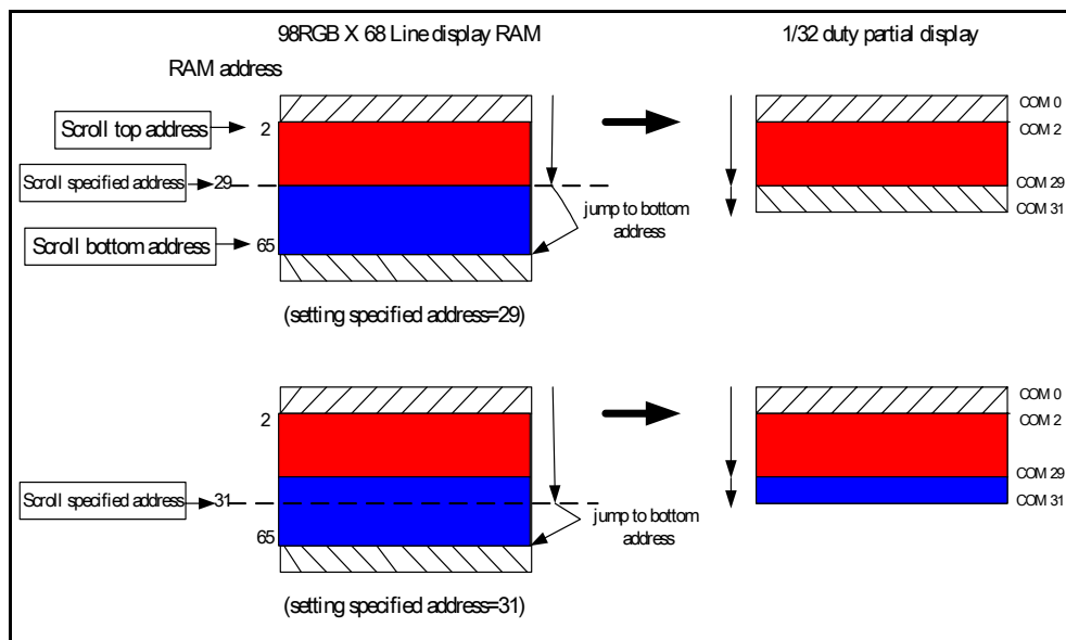
Figure 7-22b An Example of Scroll Bottom Address Settings in a Scrolling Area
