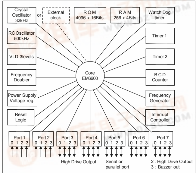
Figure 1. Architecture
