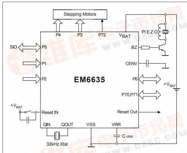
Figure 2. Typical application
