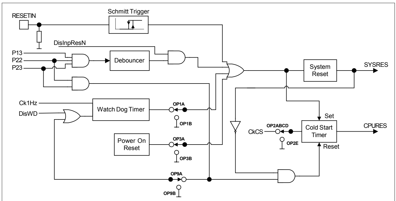
Fig.4: Reset Structure
