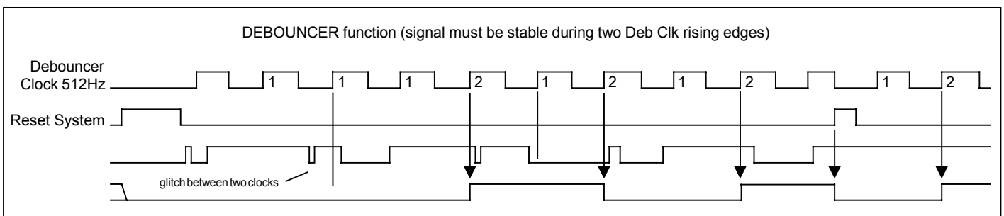
Fig.8: Debouncer function
