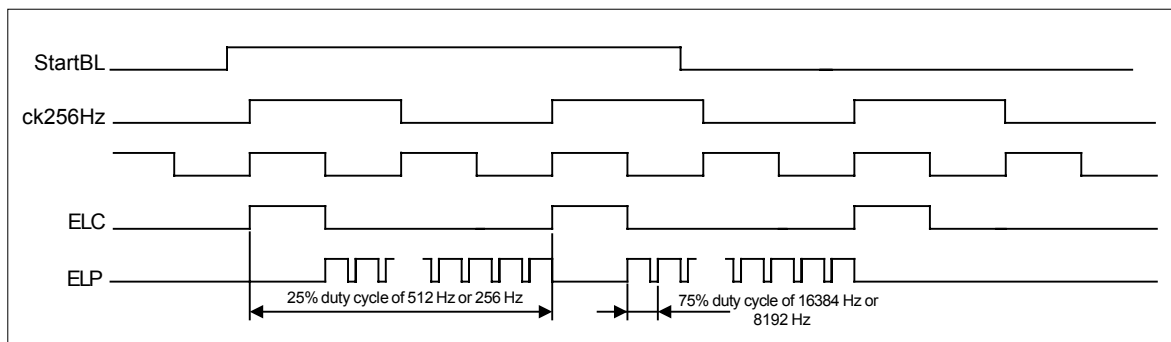
Fig. 10D: Back Light ELC and ELP signals in case where ELC is 256 Hz based.
