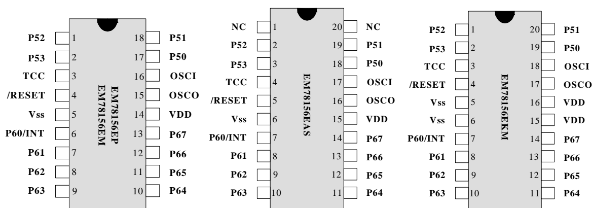
Fig. 1 Pin Assignment
