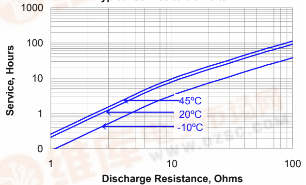
TEMPERATURE EFFECTS Typical Service to 0.8 Volts
