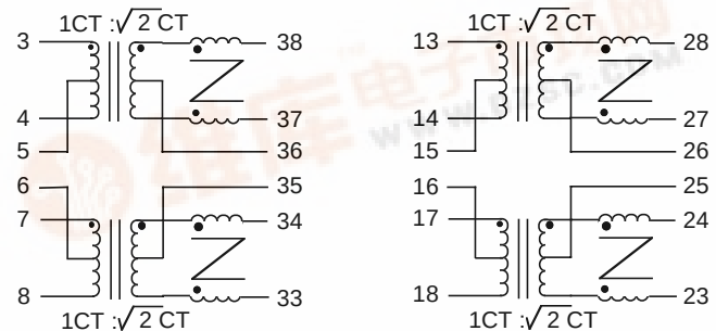
Transmit Channels
