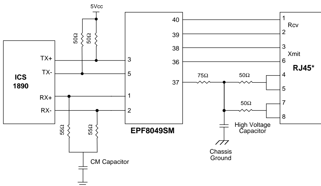
Typical Application Circuit for UTP (only one port shown)
