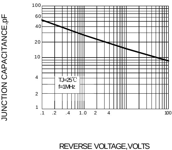
FIG.2 -- JUNCTION CHARACTERISTICS
