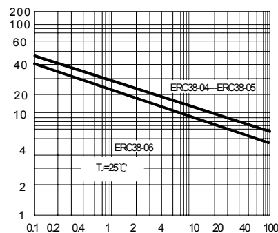
FIG.3-TYPICAL JUNCTION CAPACITANCE
