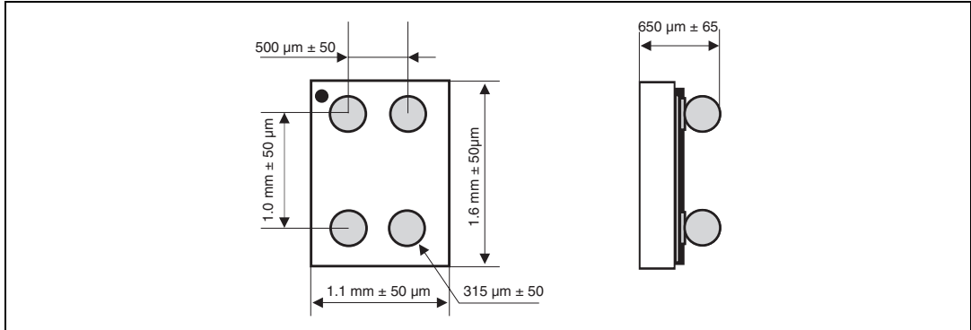
Figure 25. Flip-Chip dimensions
