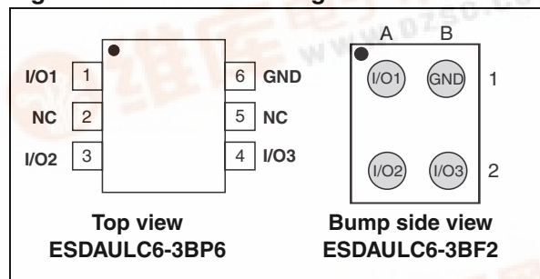
Figure 2. Pin configuration
