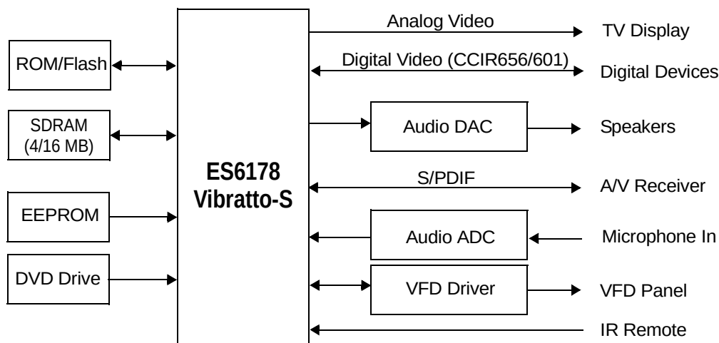
Figure 2 ES6178 Vibratto-S System Block Diagram
