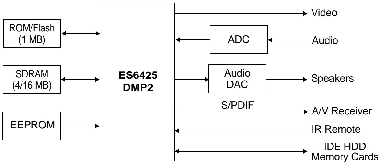
Figure 2 ES6425 System Block Diagram
