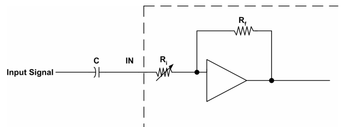
Figure 30. Input Resistor
