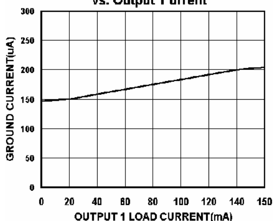
Ground Current vs. Output 1 current
