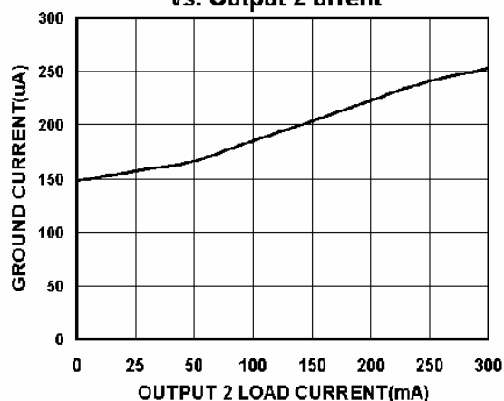
Ground Current vs. Output 2 current
