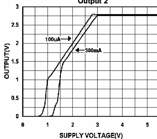
Dropout Characteristics Output 2
