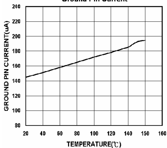
Ground Pin Current
