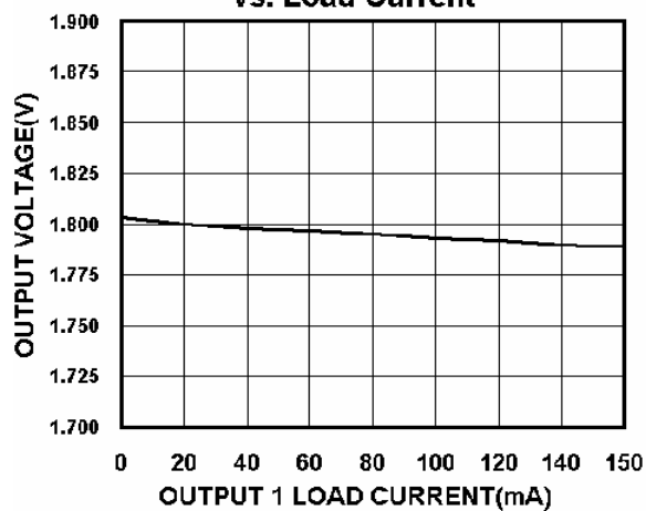
Output Voltage 1 vs. Load Current
