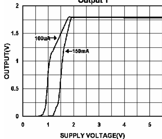
Dropout Characteristics Output 1
