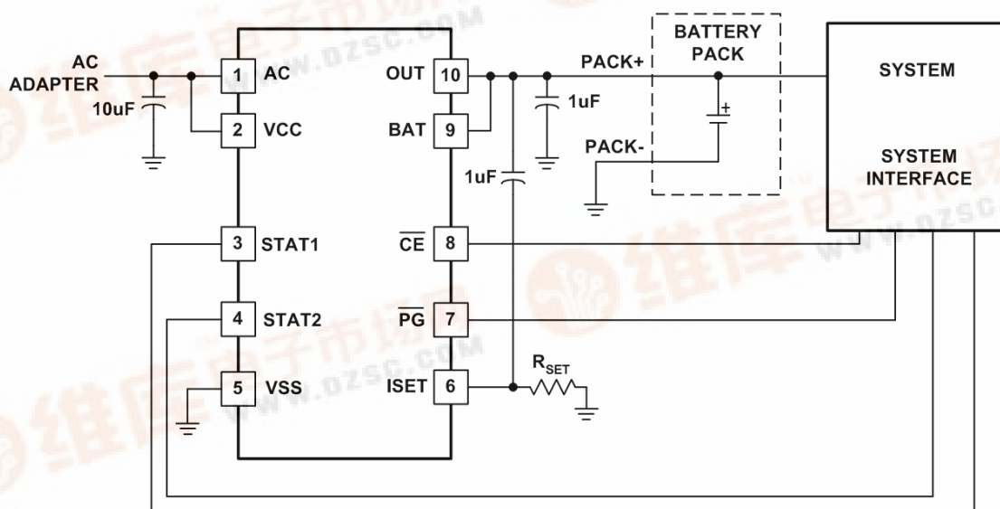
Figure 1. EUP8010B
