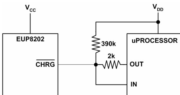
Figure 6. Microprocessor Interface
