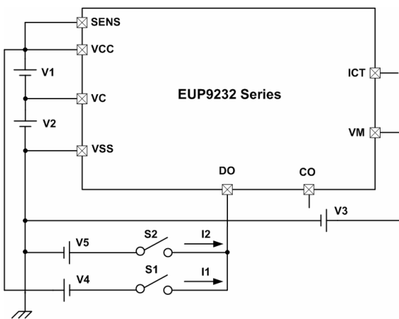
Test Circuit 3
