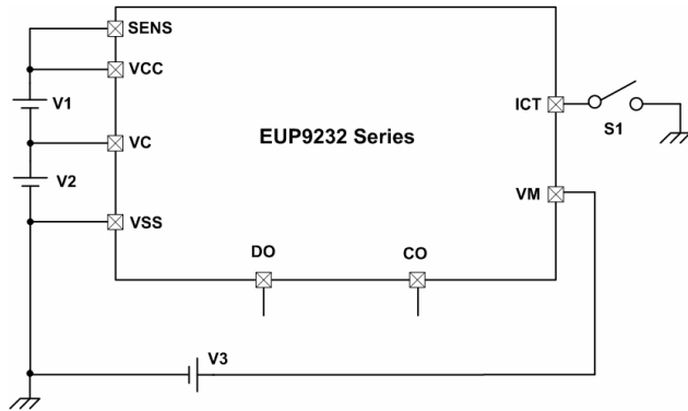
Test Circuit 1
