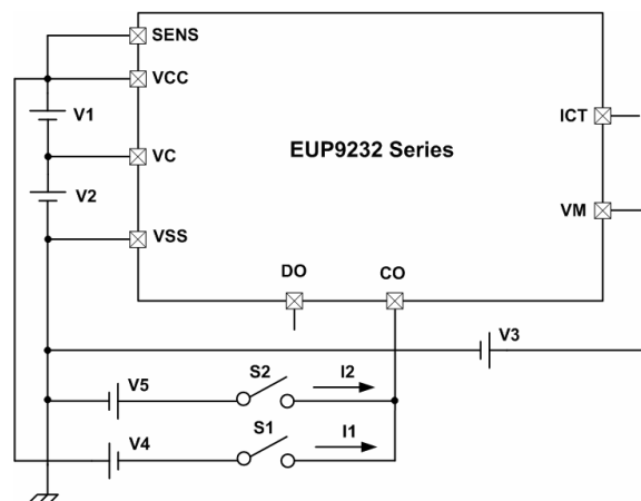
Test Circuit 4
