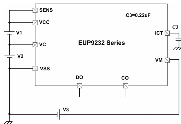
Test Circuit 5
