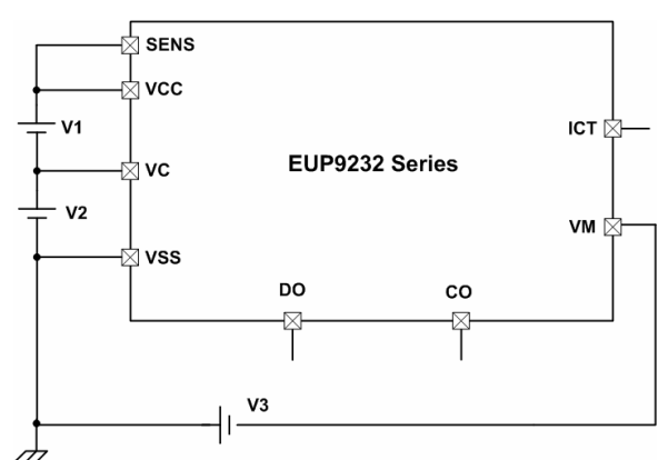
Test Circuit 6
