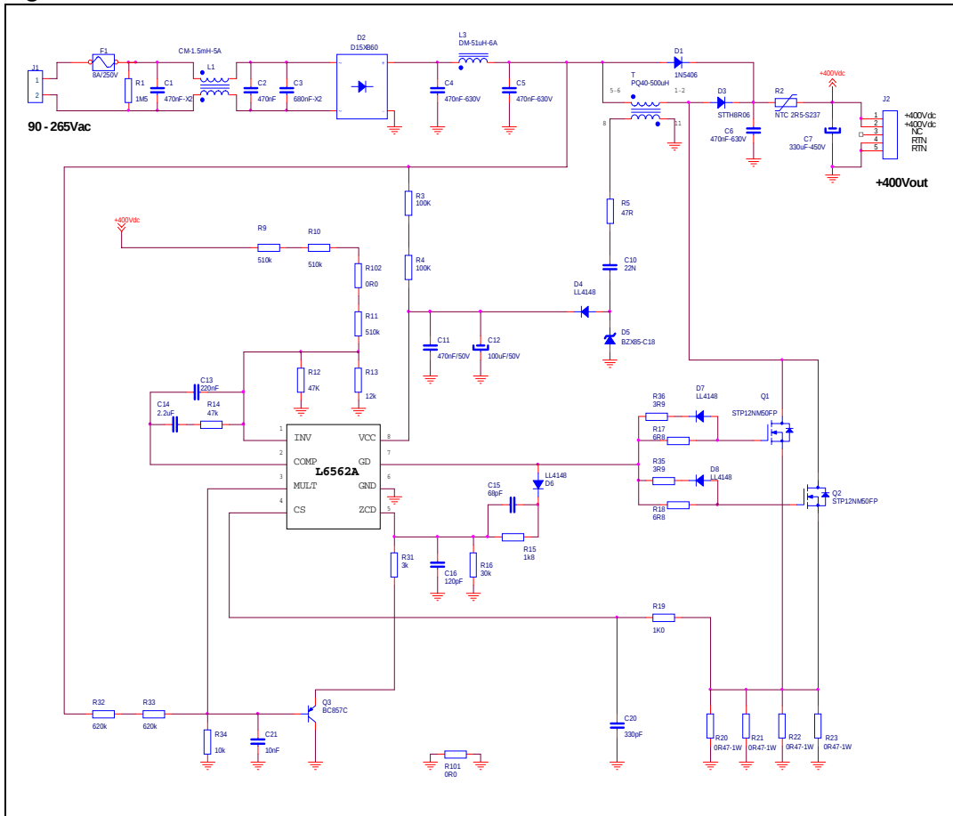
Figure 1. EVL6562A-400W schematic
