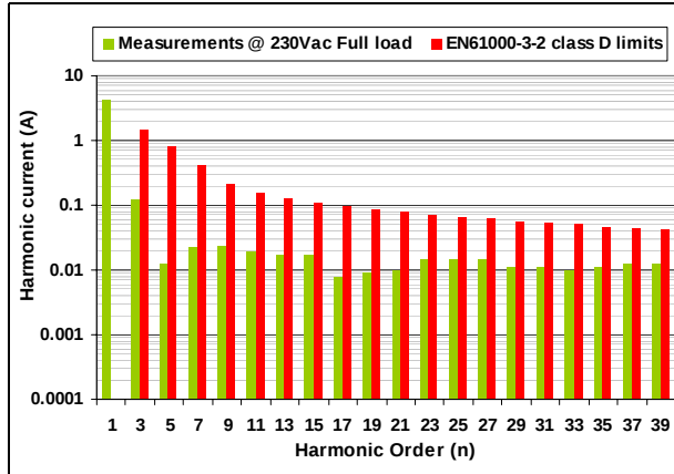
Figure 3. EVL6562A-400W compliance to EN61000-3-2 standard @full load
