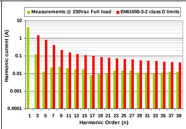
Figure 4. EVL6562A-400W compliance to JEIDA-MITI standard @full load
