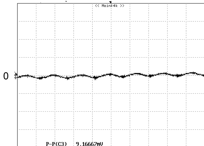
Figure 12: Input reflected ripple current, i_s , through a 12\mu\text{H} source inductor at nominal input voltage and rated load current (20 mA/div, 2µs/div)
