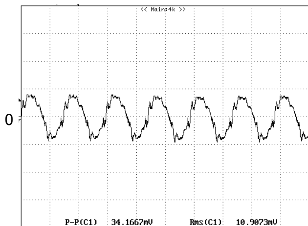
Figure 14: Output voltage ripple at nominal input voltage and rated load current ( I_o=5\text{A} ) (20 mV/div, 2µs/div) Load capacitance: 1\mu\text{F} ceramic capacitor and 10\mu\text{F} tantalum capacitor. Bandwidth: 20 MHz. Scope measurements should be made using a BNC cable (length shorter than 20 inches). Position the load between 51 mm to 76 mm (2 inches to 3 inches) from the module
