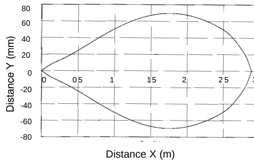
E3F2-R2R□□-4□ (Polarized, retroreflective)
