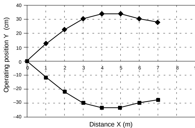
E3F2-7□□-4□ (Through-beam)
