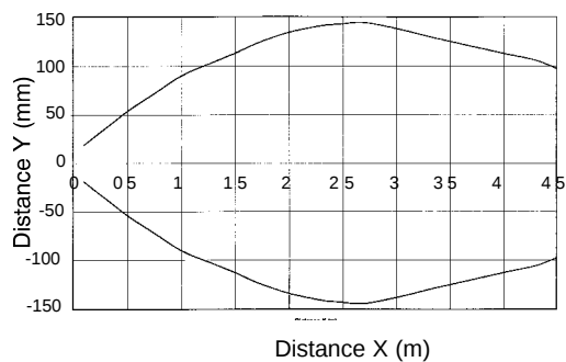
E3F2-7□□-4□ (Through-beam)
