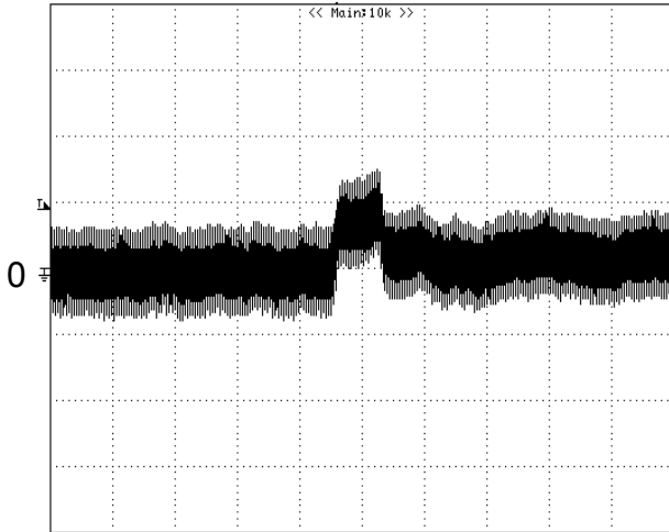
Figure 8: Output voltage response to step-change in load current (75%-50% of I_o, \max ; di/dt = 0.1A/\mu s ). Load cap: 10\mu F , tantalum capacitor and 1\mu F ceramic capacitor. Trace: V_{out} (20mV/div, 100us/div), Scope measurement should be made using a BNC cable (length shorter than 20 inches). Position the load between 51 mm to 76 mm (2 inches to 3 inches) from the module..
