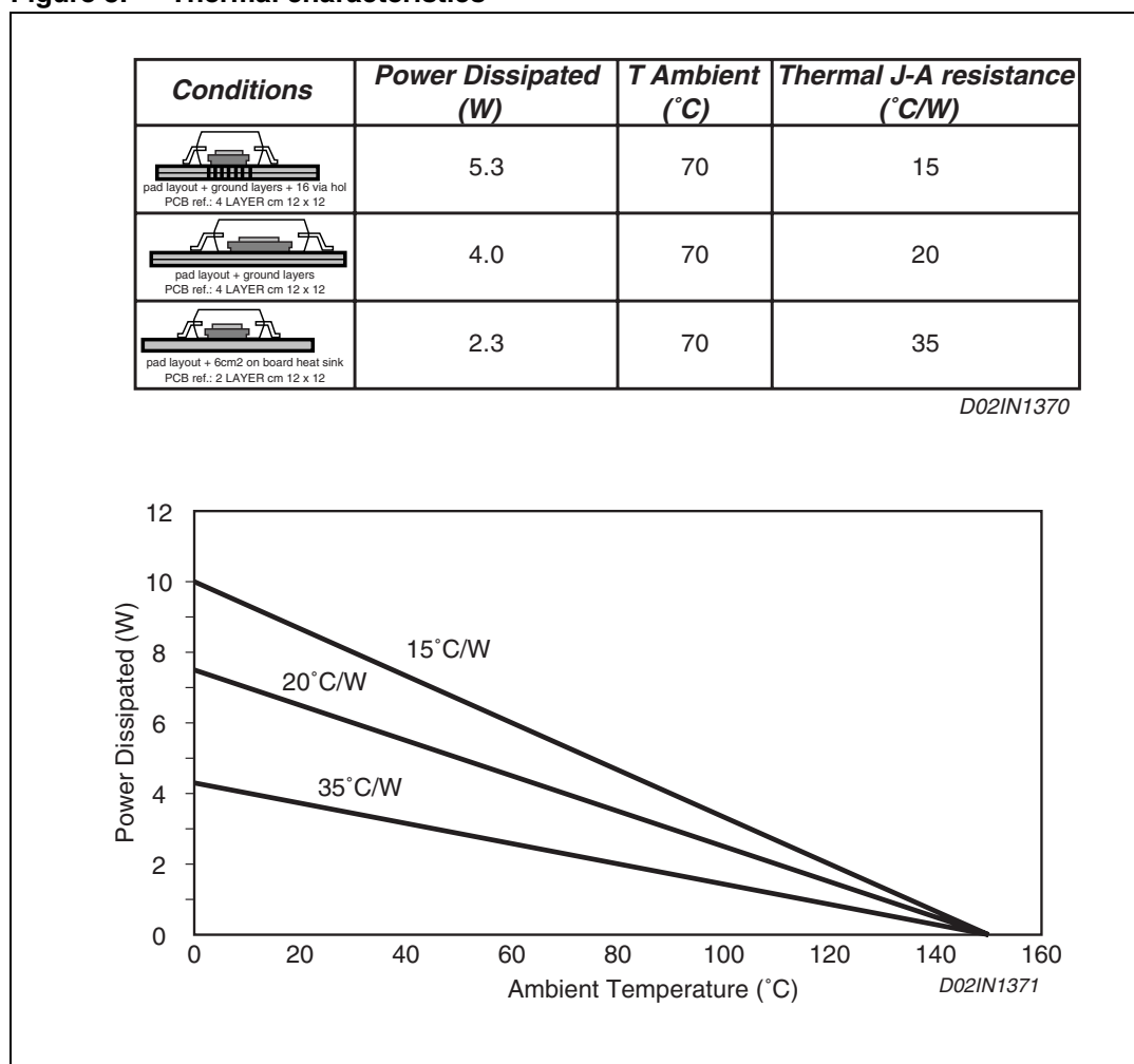
Figure 3. Thermal characteristics
