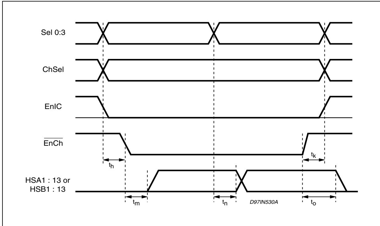
Figure 14. Sequence of Shift Register Data Loading
