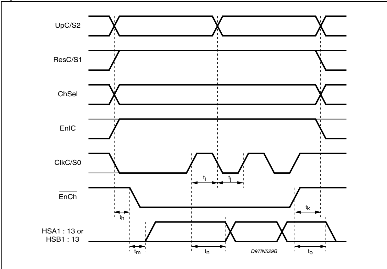
Figure 12. Mode Counter
