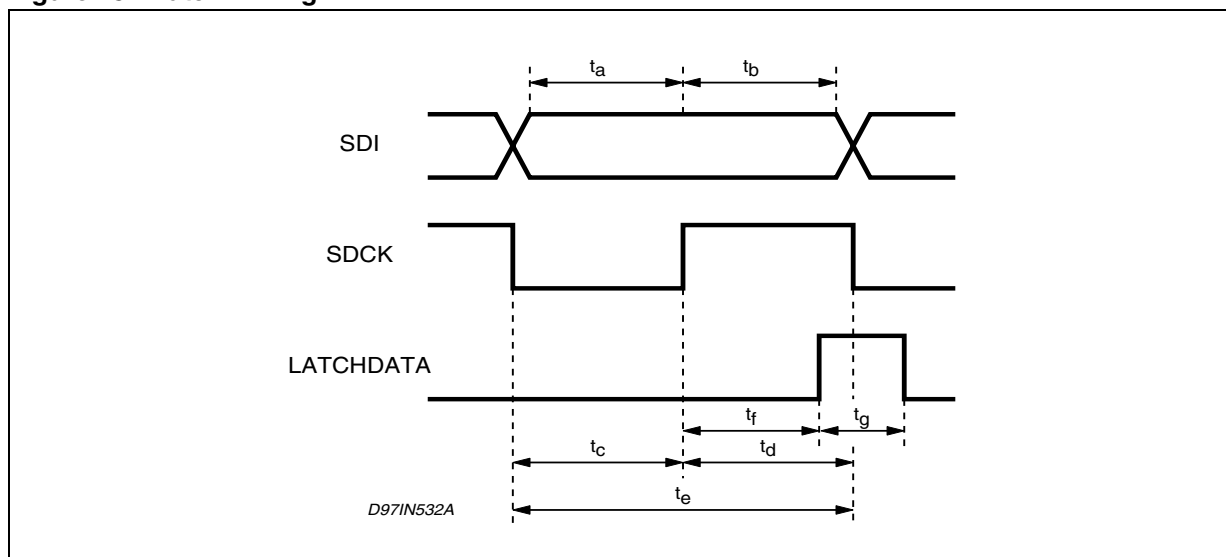
Figure 15. Latch Timing
