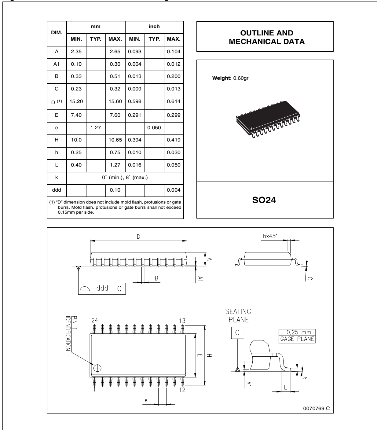
Figure 17. SO24 Mechanical Data & Package Dimensions
