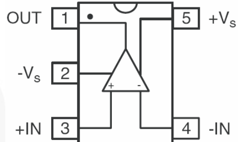
Figure 4. FAN4147 SC70
