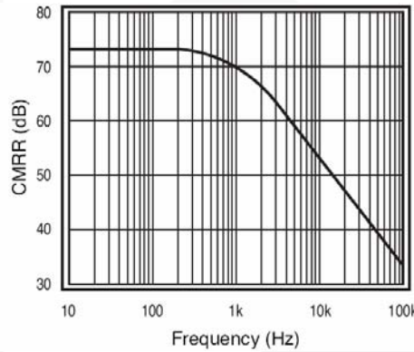
Figure 17. CMRR V_S=5V
