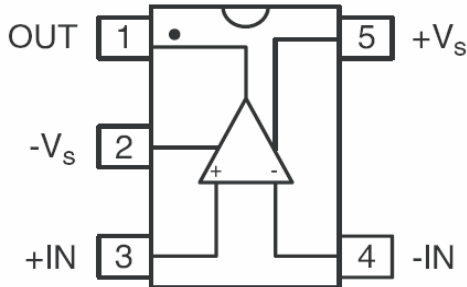
Figure 3. FAN4174 SOT23
