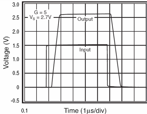
Figure 24. Overdrive Recovery
