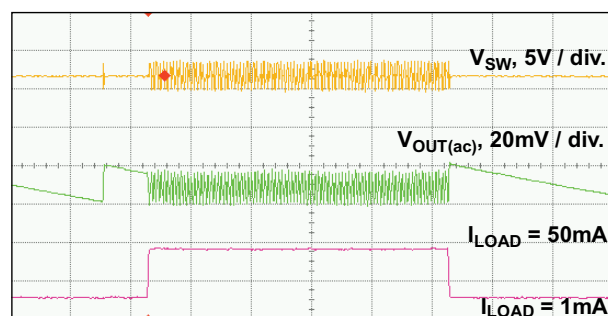
Figure 25. Fast Load Transient in DCM
