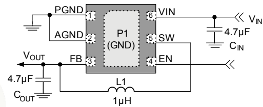
Figure 2. MLP (top view)
