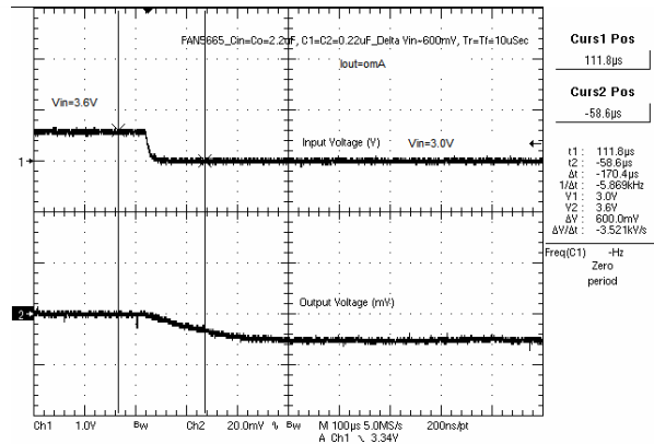
Figure 38. Line Transient 600mV Falling
