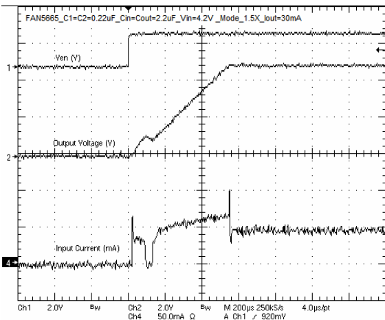
Figure 27. Start-up at I_{OUT} = 30\text{mA} in 1.5x Mode
