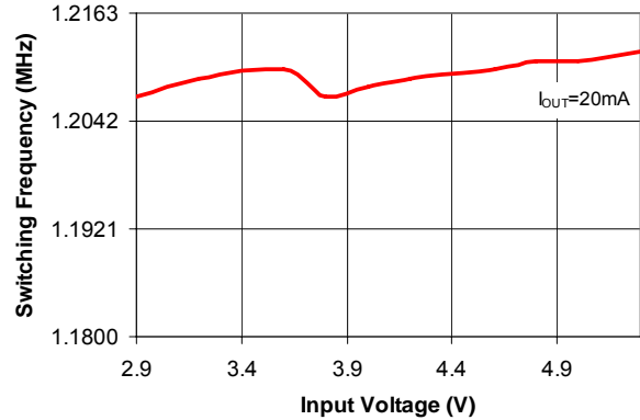
Figure 4. Heavy-Load Switching Frequency vs. Input Voltage
