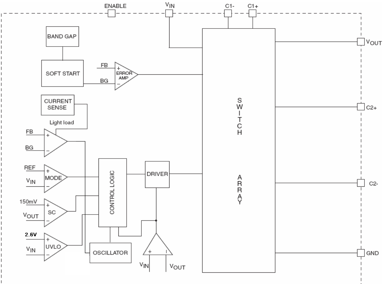
Figure 39. Block Diagram
