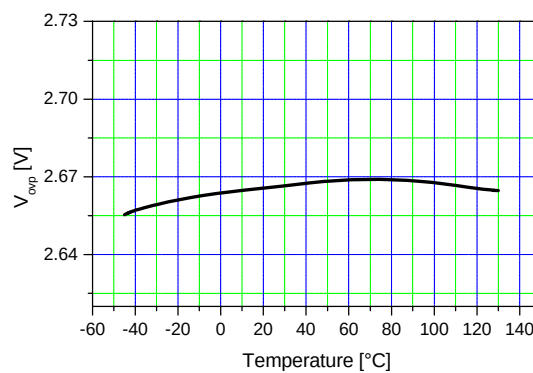
Figure 29. OVP Threshold Voltage vs. Temp.
