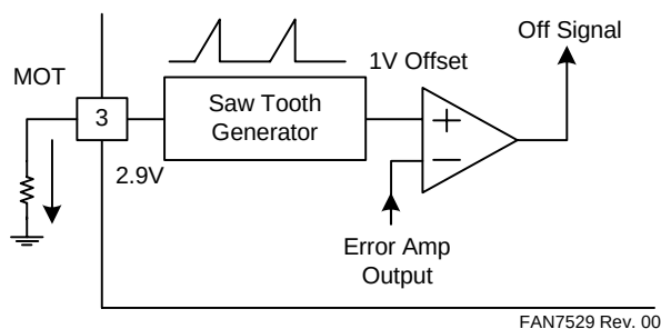
Figure 35. Sawtooth Generator Block
