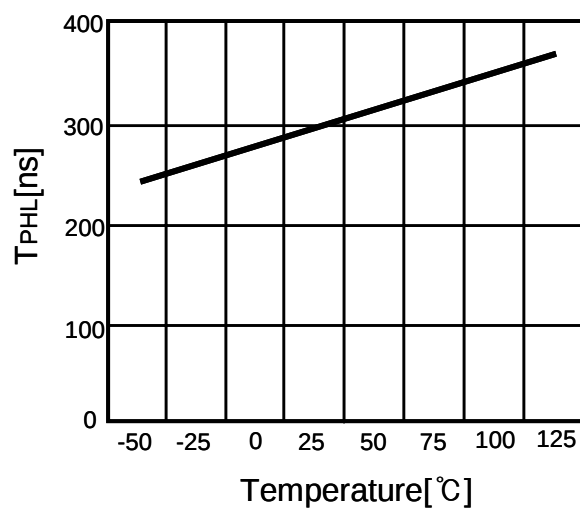
4. Temperature vs. T PHL
