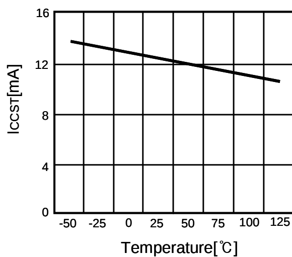
2. Temperature vs. Iccst
