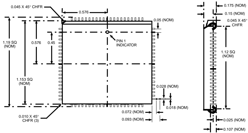
Figure 6. FAS216/216U 84-Pin PLCC Mechanical Drawings
