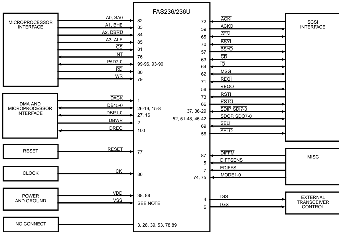
Figure 5. FAS236/236U Functional Signal Grouping
