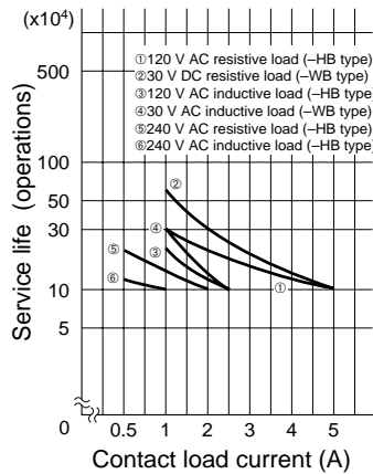
Life curve (5 A type)
