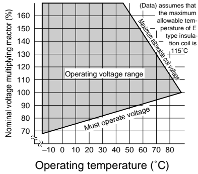
Range of operation temperature and voltage E type [0.36 W type]
