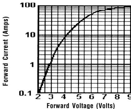
Forward Characteristics
