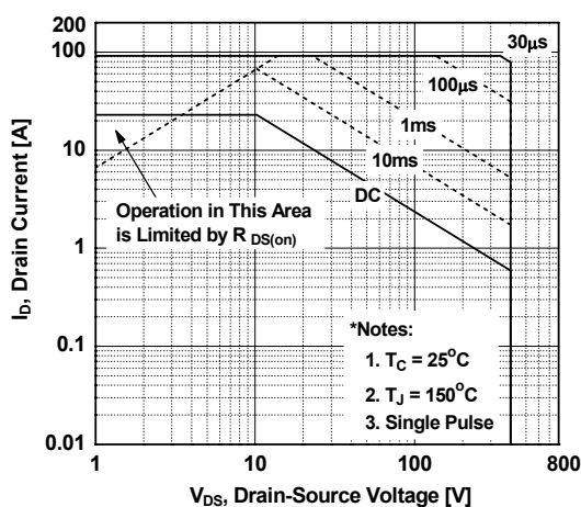
Figure 8. Maximum Safe Operating Area vs. Temperature
