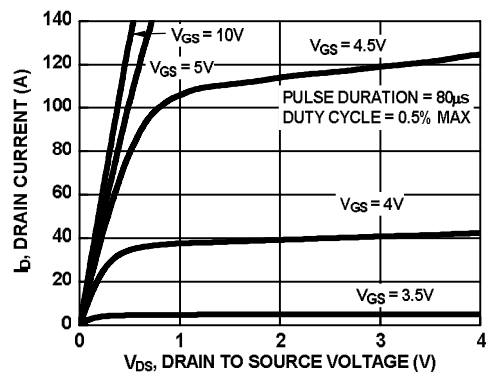
Figure 8. Saturation Characteristics
