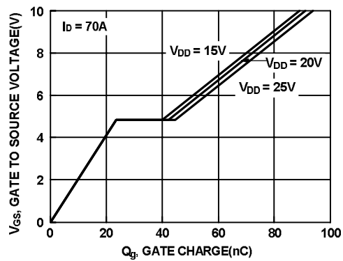
Figure 14. Gate Charge vs Gate to Source Voltage
