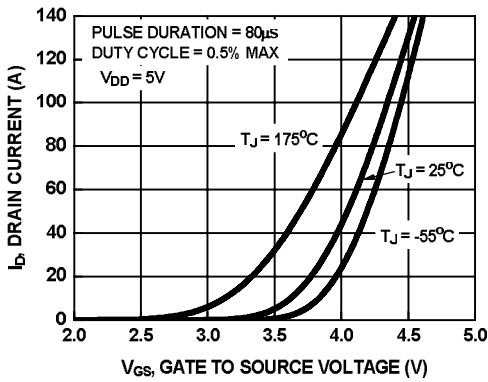
Figure 7. Transfer Characteristics
