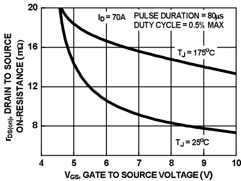
Figure 9. On-Resistance vs Gate to Source Voltage
