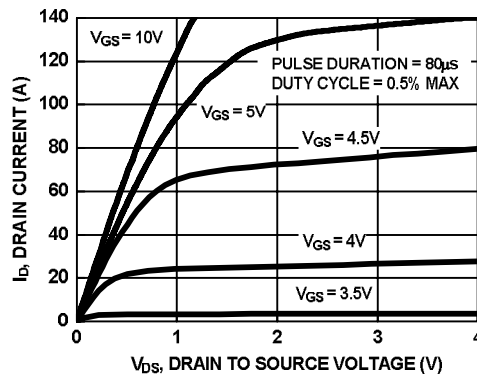
Figure 8. Saturation Characteristics
