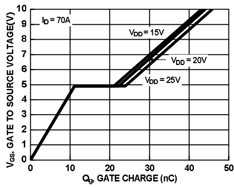
Figure 14. Gate Charge vs Gate to Source Voltage
