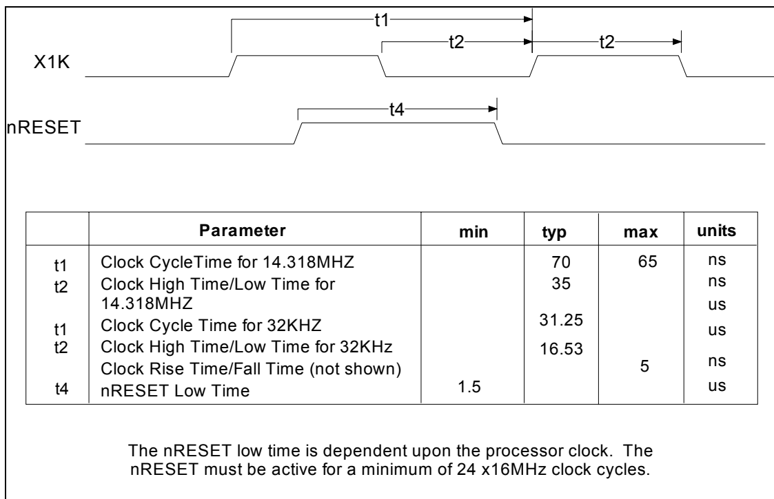
FIGURE 7 - CLOCK TIMING
