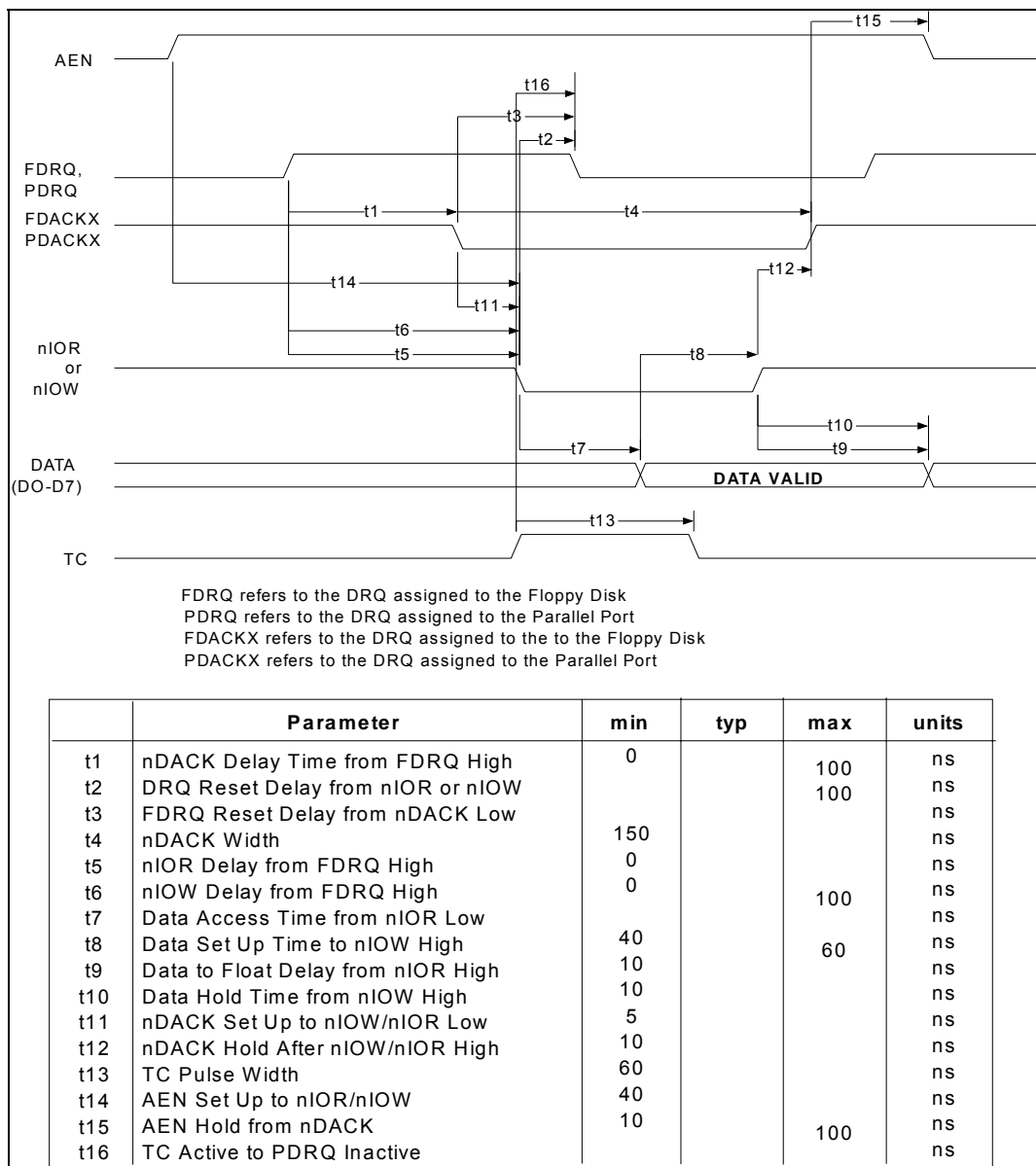
FIGURE 6 - DMA TIMING
