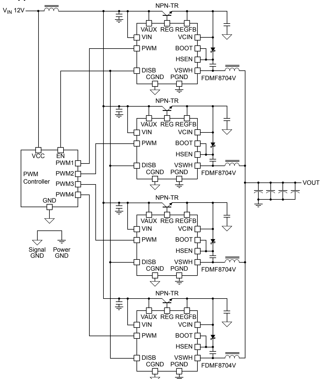
Figure 17. Typical Application
