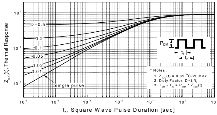
Figure 11-1. Transient Thermal Response Curve - FDP14N30
