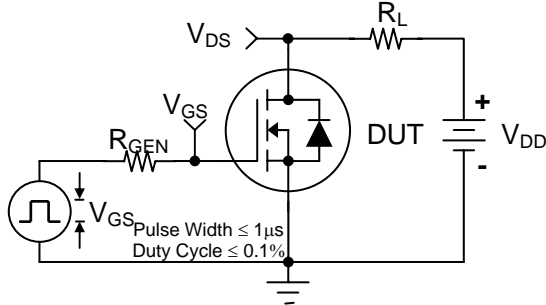
Figure 30. Switching Time Test Circuit
