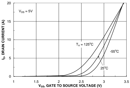
Figure 16. Transfer Characteristics.
