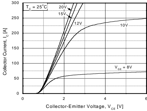
Figure 3. Saturation Voltage
