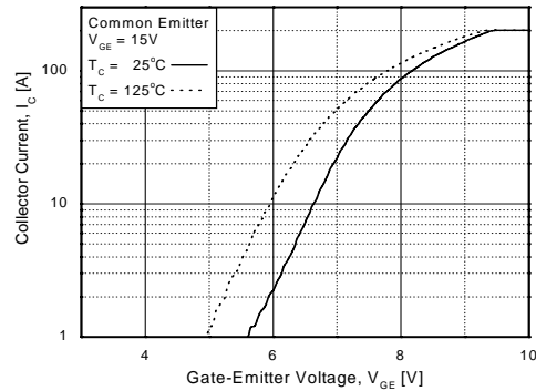
Figure 4. Transfer Characteristics
