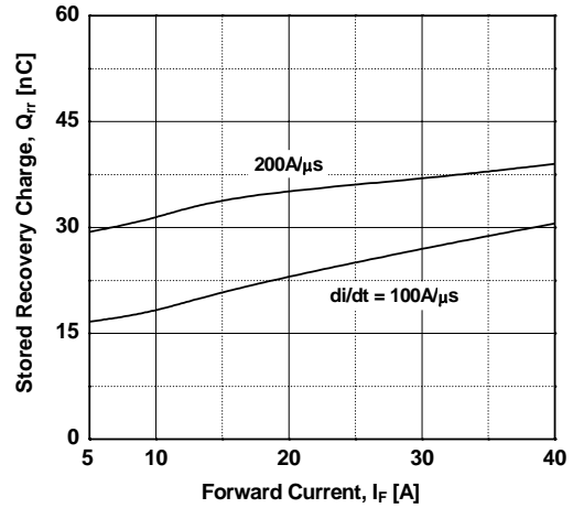
Figure 18. Stored Charge
