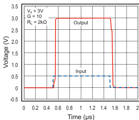
Figure 28. Overdrive Recovery
