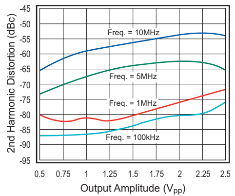
Figure 16. HD2 vs. V_{OUT} (3V)
