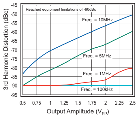
Figure 17. HD3 vs. V_{OUT} (3V)
