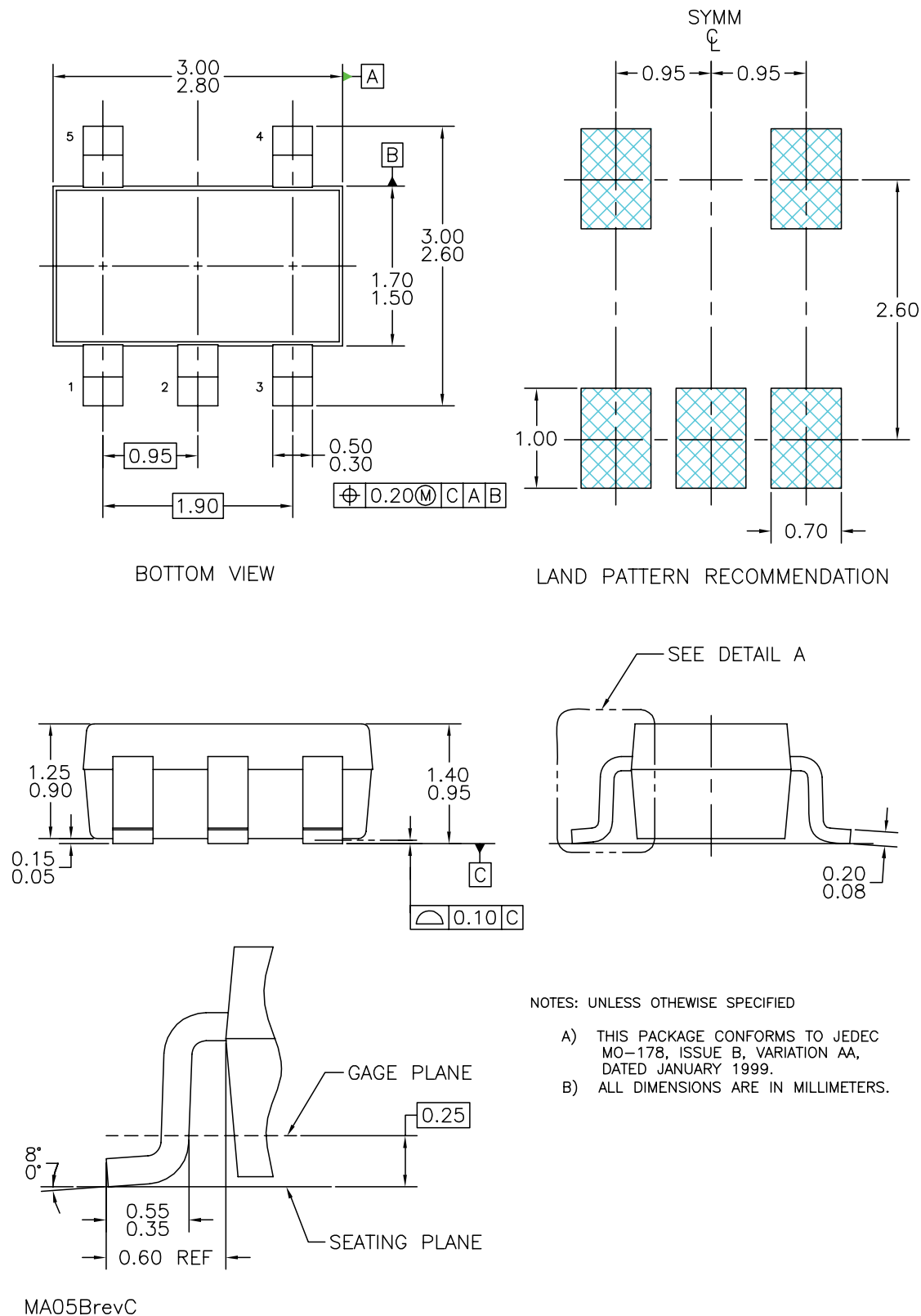
Figure 35. SOT23-5 Package
