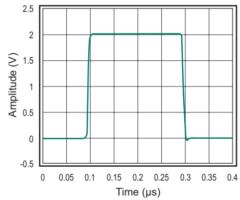
Figure 23. Pulse Response (3V)
