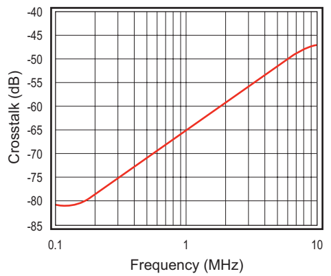
Figure 22. Crosstalk vs. Frequency (3V)
