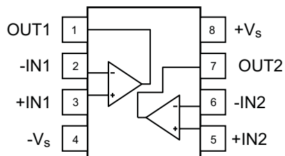
Figure 2. FHP3232 SOIC
