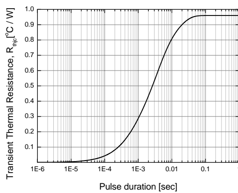
Figure 6. Thermal Resistance
