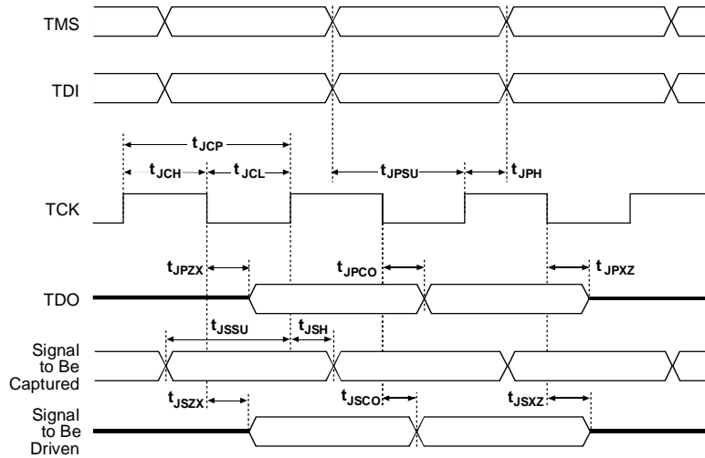
Figure 16. JTAG Waveforms
