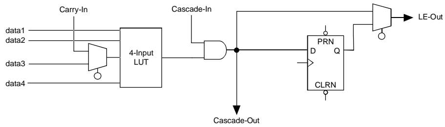
Figure 7. LE Operating Modes
