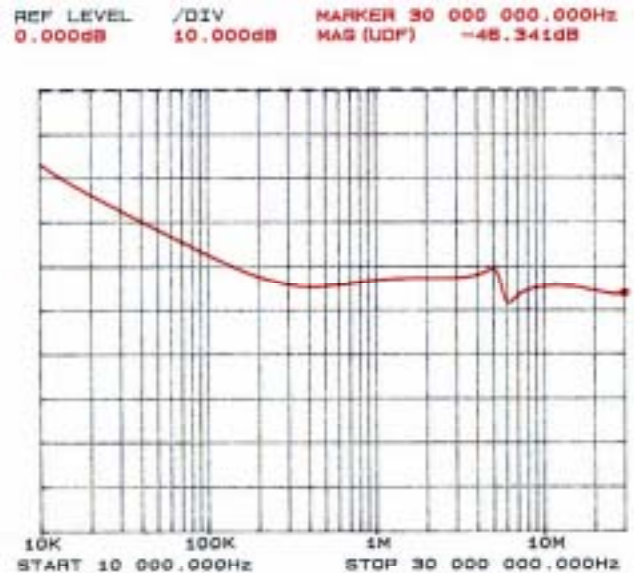
Figure 2: Typical differential-mode insertion loss in a 50 ohm circuit
