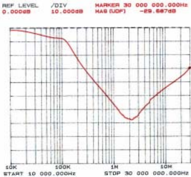
Figure 1: Typical common-mode insertion loss in a 50 ohm circuit
