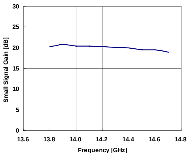
SMALL SIGNAL GAIN vs. FREQUENCY Vdd=10V, Vgg=-5V
