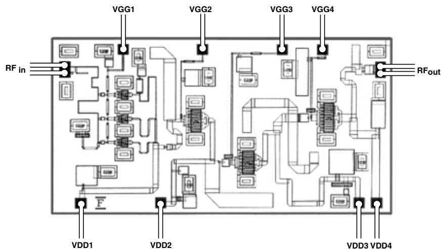
BONDING LAYOUT
