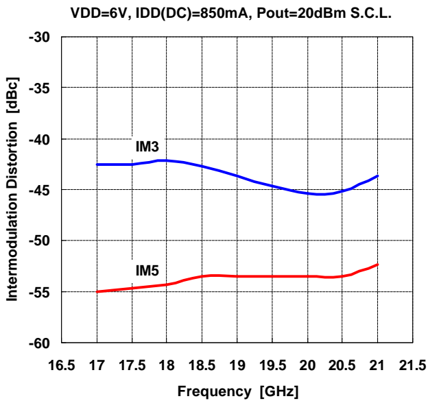
IMD vs. Frequency
