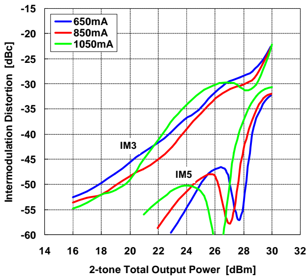
IMD vs. Output Power by Drain Current
